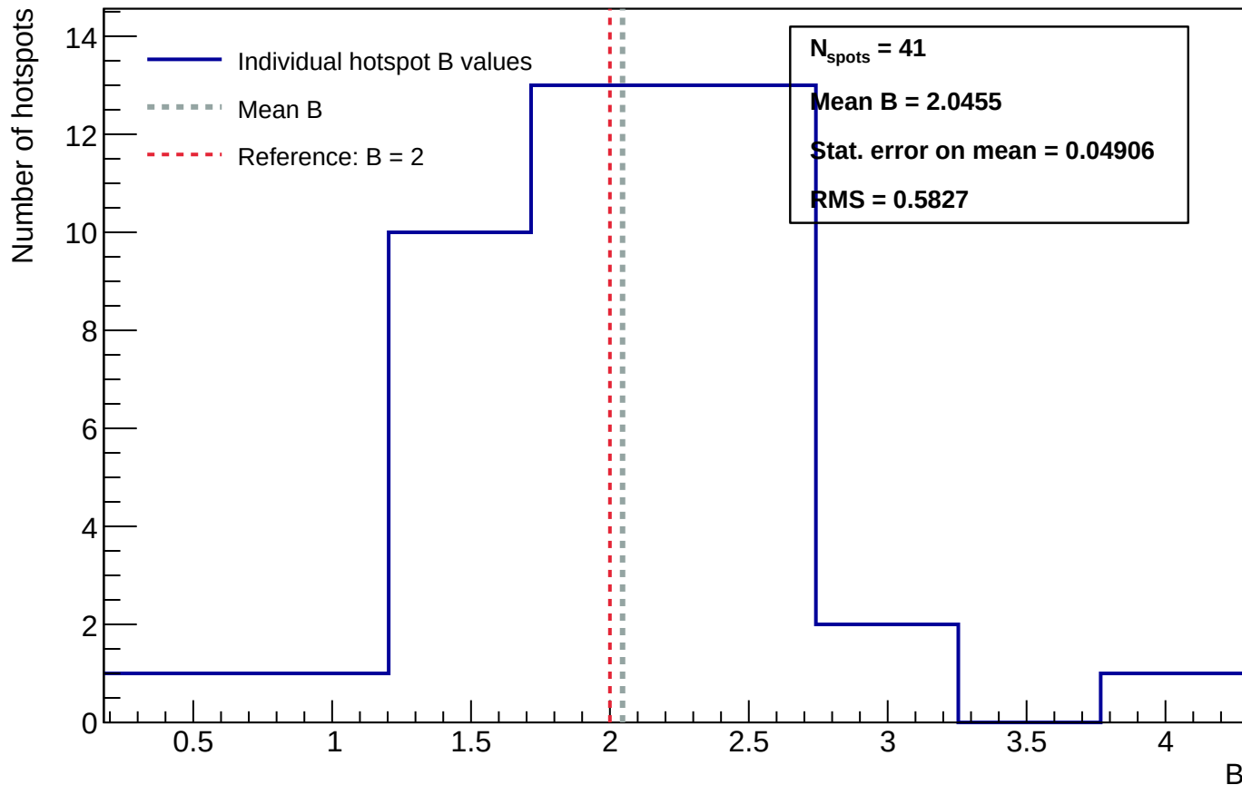
Sensor A1 - Distribution of power-law exponent B - annealing_T=125_h=5
