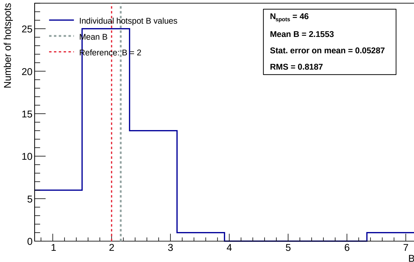
Sensor A1 - Distribution of power-law exponent B - annealing_T=75_h=25
