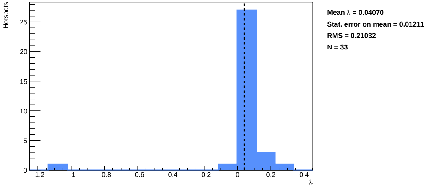
A1_v=5_annealing_T=150_h=25 - Distribution of fitted \lambda - annealing_T=150_h=25
