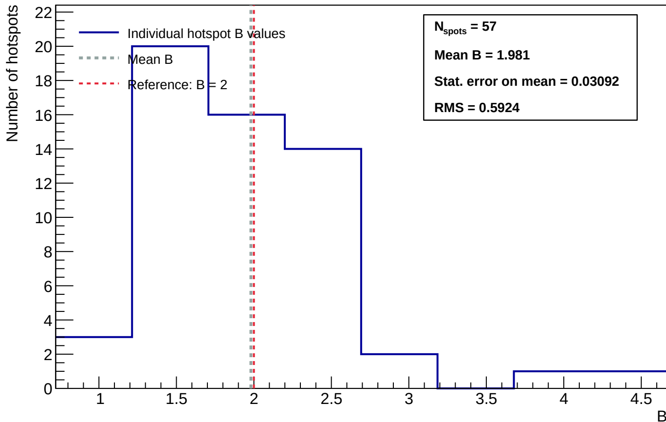
Sensor B1 - Distribution of power-law exponent B - annealing_T=100_h=25
