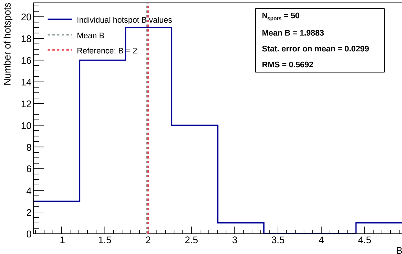
Sensor B1 - Distribution of power-law exponent B - annealing_T=100_h=5
