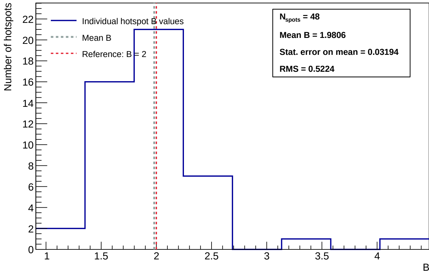
Sensor B1 - Distribution of power-law exponent B - annealing_T=125_h=5
