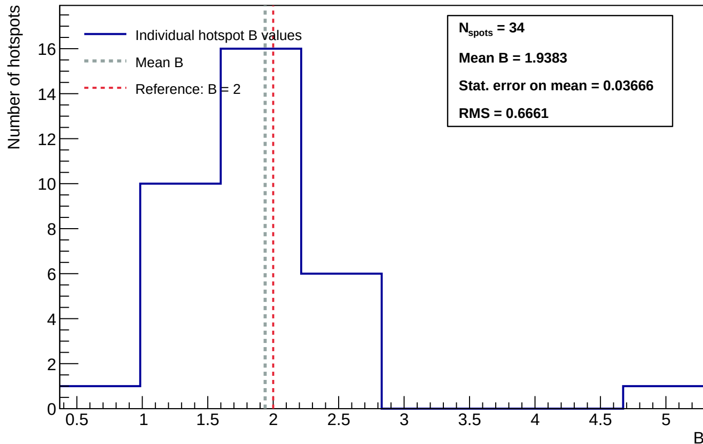
Sensor B1 - Distribution of power-law exponent B - annealing_T=150_h=25
