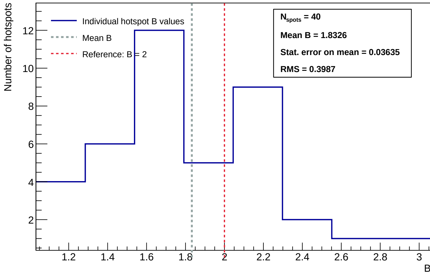
Sensor B1 - Distribution of power-law exponent B - annealing_T=150_h=5
