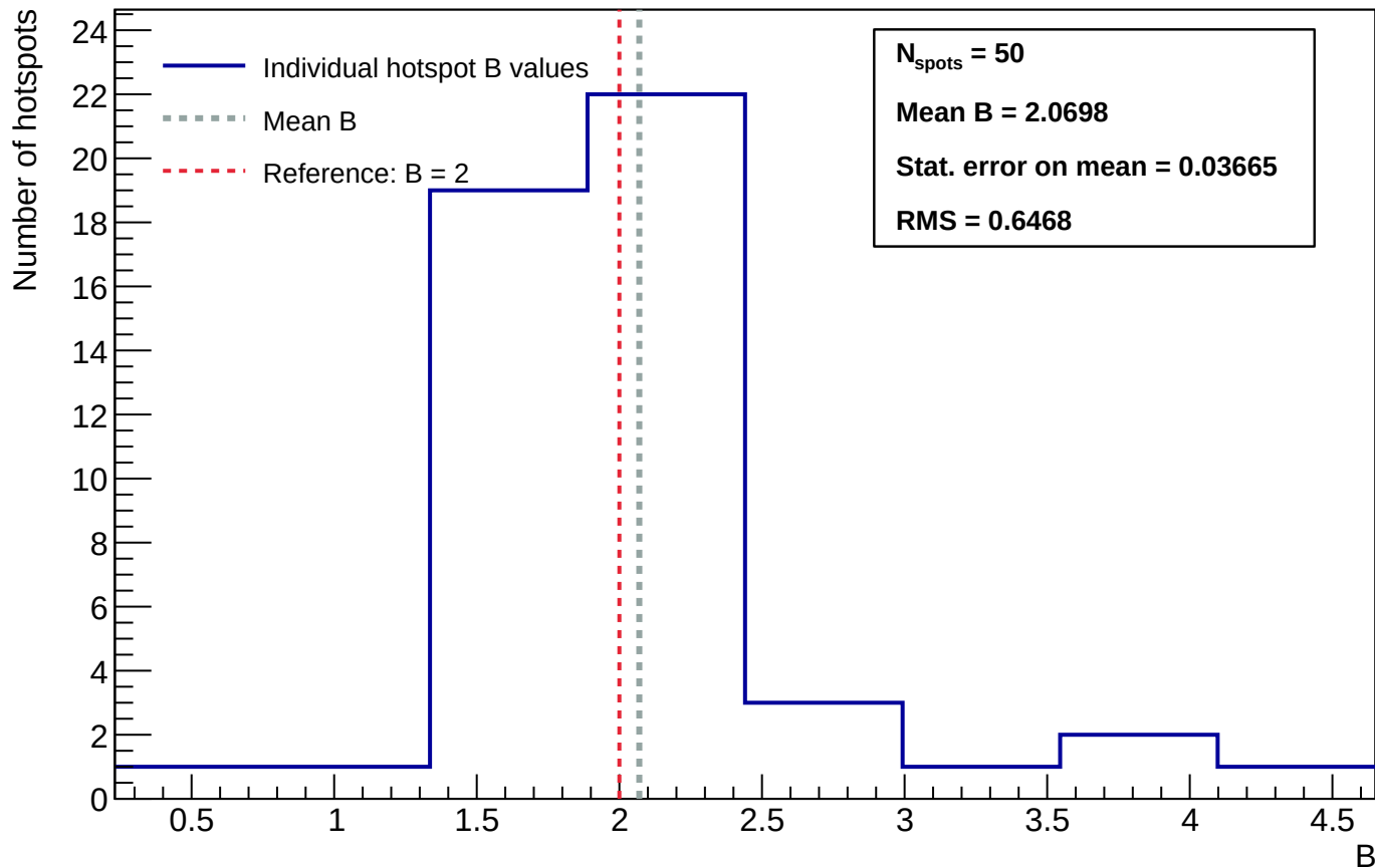
Sensor B1 - Distribution of power-law exponent B - annealing_T=75_h=25
