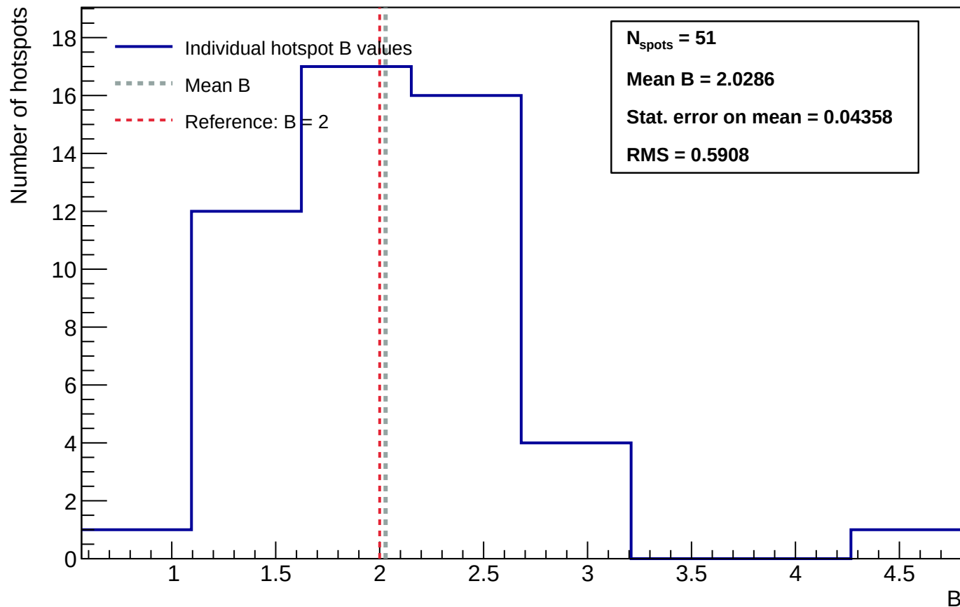
Sensor B1 - Distribution of power-law exponent B - annealing_T=75_h=5
