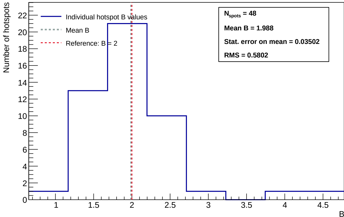
Sensor B1 - Distribution of power-law exponent B - before_annealing
