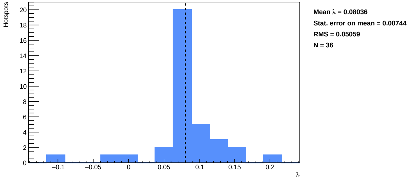
B1_v=3_annealing_T=150_h=5 - Distribution of fitted \lambda - annealing_T=150_h=5
