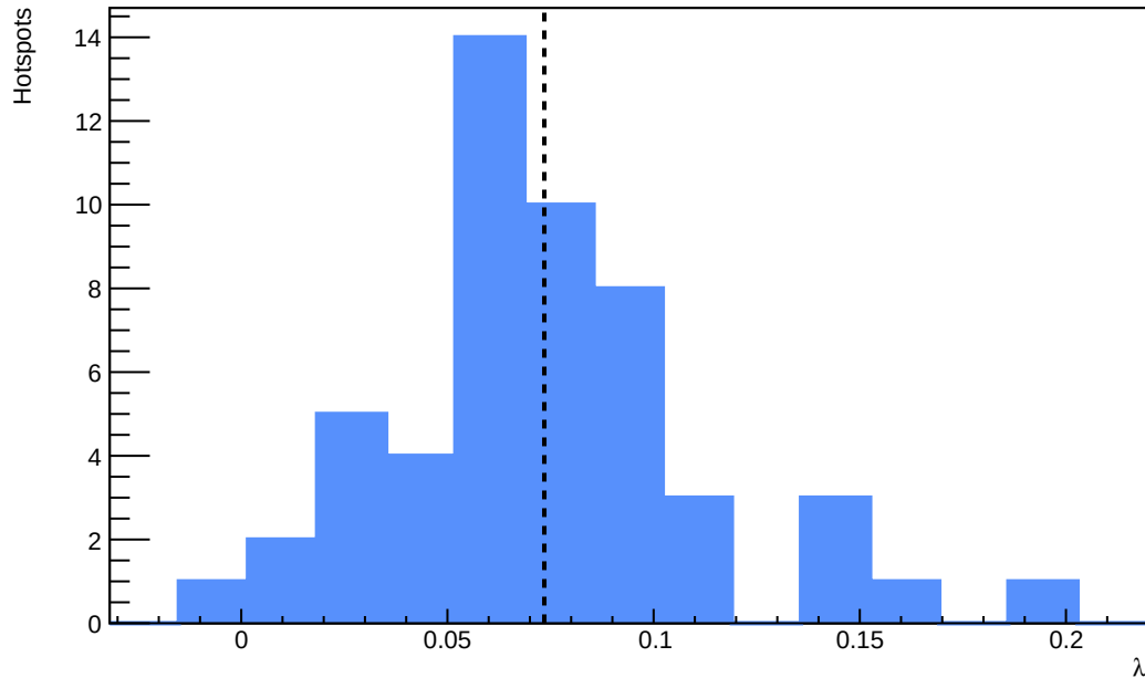
B1_v=3_annealing_T=75_h=25 - Distribution of fitted \lambda - annealing_T=75_h=25
