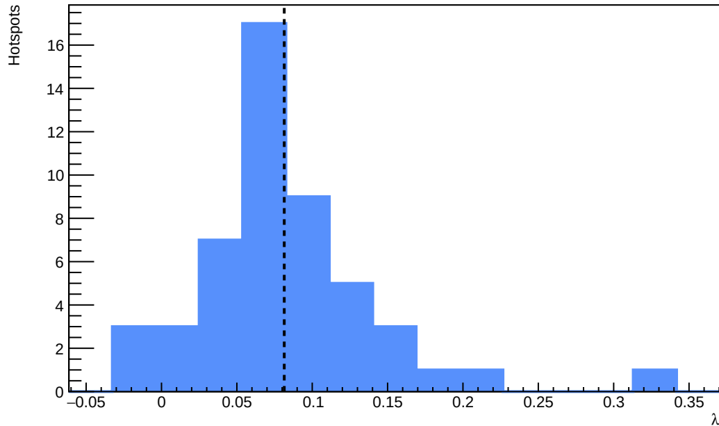
B1_v=3_annealing_T=75_h=5 - Distribution of fitted \lambda - annealing_T=75_h=5
