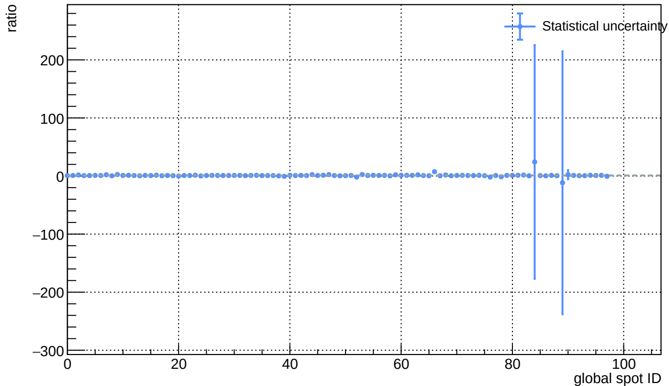
Sensor A1, T = 20 C - L(\text{ann\_75C\_25h}) / L(\text{before\_annealing})
