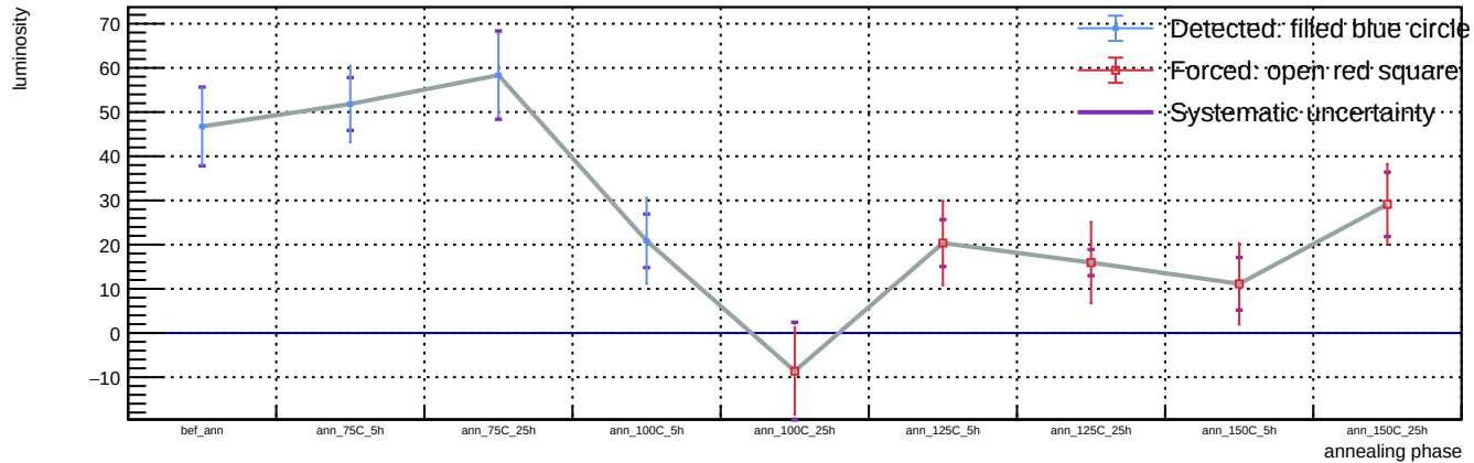
Sensor A1, T = 20 C, representative v = 58.3 V (max available) - Spot 11: luminosity vs phase
