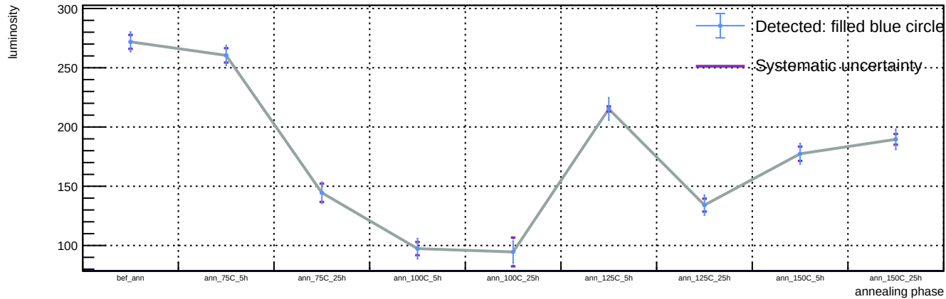
Sensor A1, T = 20 C, representative v = 58.3 V (max available) - Spot 17: luminosity vs phase
