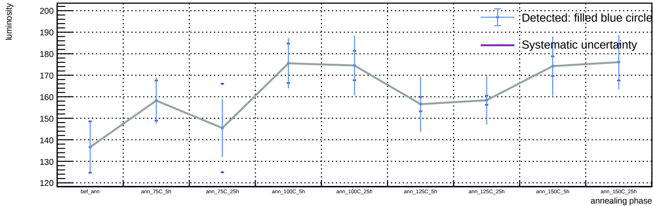
Sensor A1, T = 20 C, representative v = 58.3 V (max available) - Spot 42: luminosity vs phase
