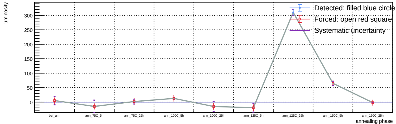
Sensor A1, T = 20 C, representative v = 58.3 V (max available) - Spot 83: luminosity vs phase
