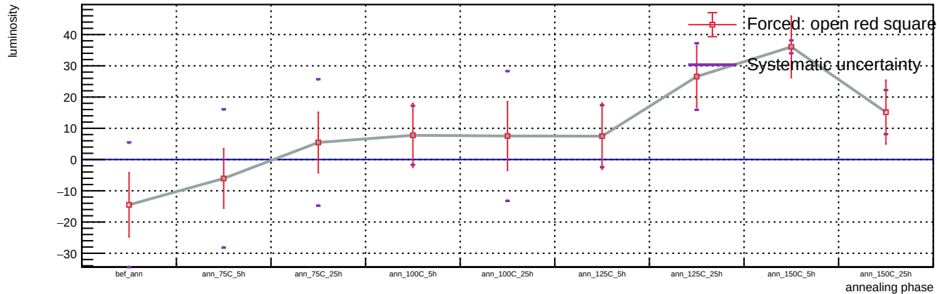
Sensor A1, T = 20 C, representative v = 58.3 V (max available) - Spot 97: luminosity vs phase
