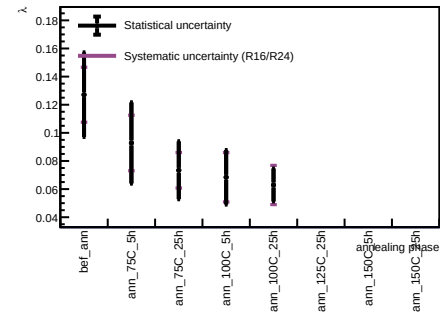
Sensor A1, v = 5 V - Spot 23
