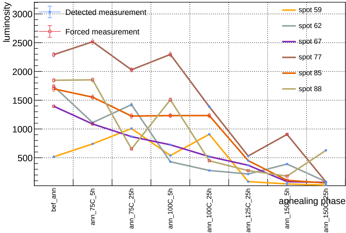
Sensor A1, v = 5 V, representative T = 23 C (max available) - luminosity vs phase - order 10^3
