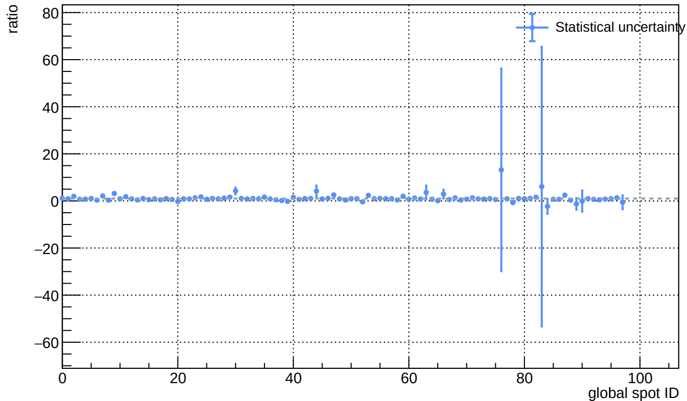
Sensor A1, v = 5\text{ V} - L(\text{ann\_75C\_25h}) / L(\text{before\_annealing})
