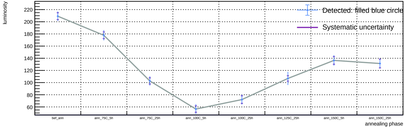
Sensor A1, v = 5 V, representative T = 23 C (max available) - Spot 17: luminosity vs phase
