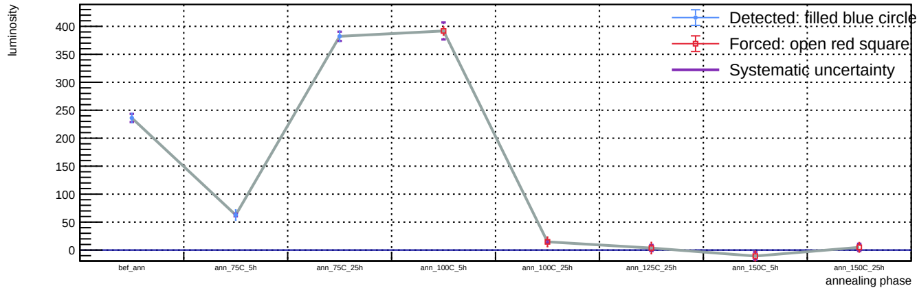
Sensor A1, v = 5 V, representative T = 23 C (max available) - Spot 35: luminosity vs phase
