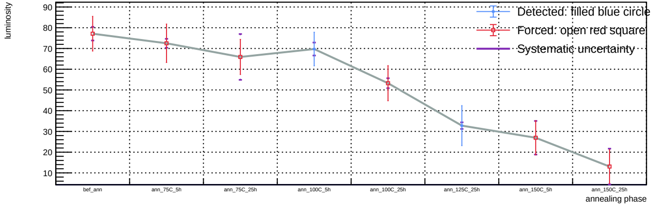
Sensor A1, v = 5 V, representative T = 23 C (max available) - Spot 36: luminosity vs phase
