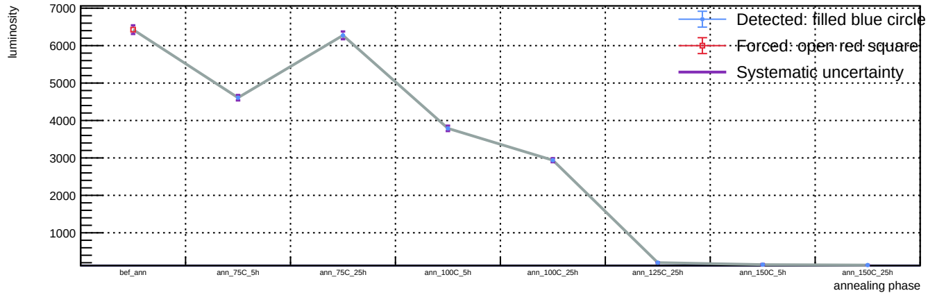
Sensor A1, v = 5 V, representative T = 23 C (max available) - Spot 54: luminosity vs phase
