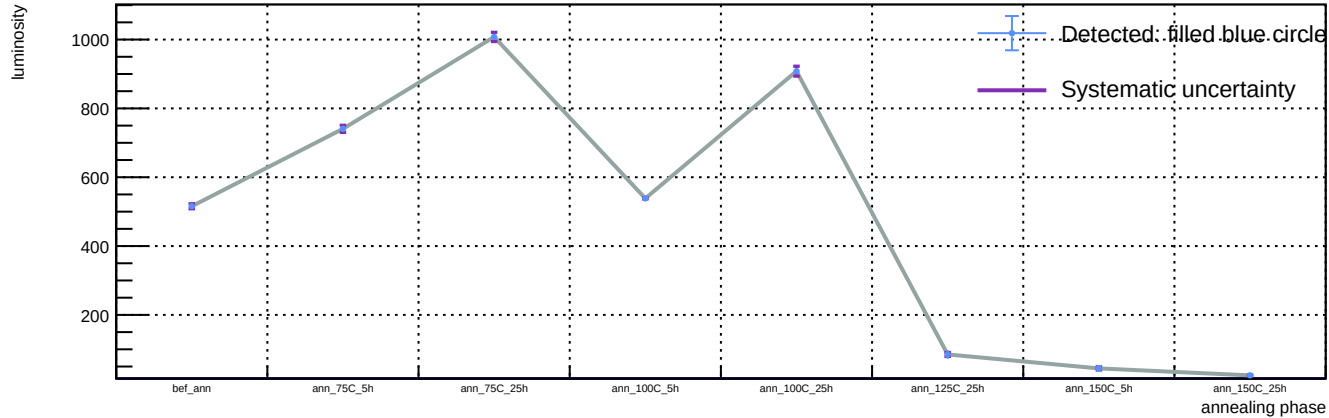
Sensor A1, v = 5 V, representative T = 23 C (max available) - Spot 59: luminosity vs phase
