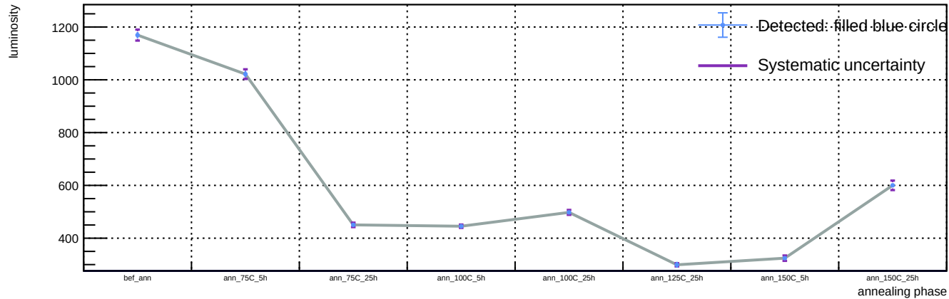
Sensor A1, v = 5 V, representative T = 23 C (max available) - Spot 6: luminosity vs phase
