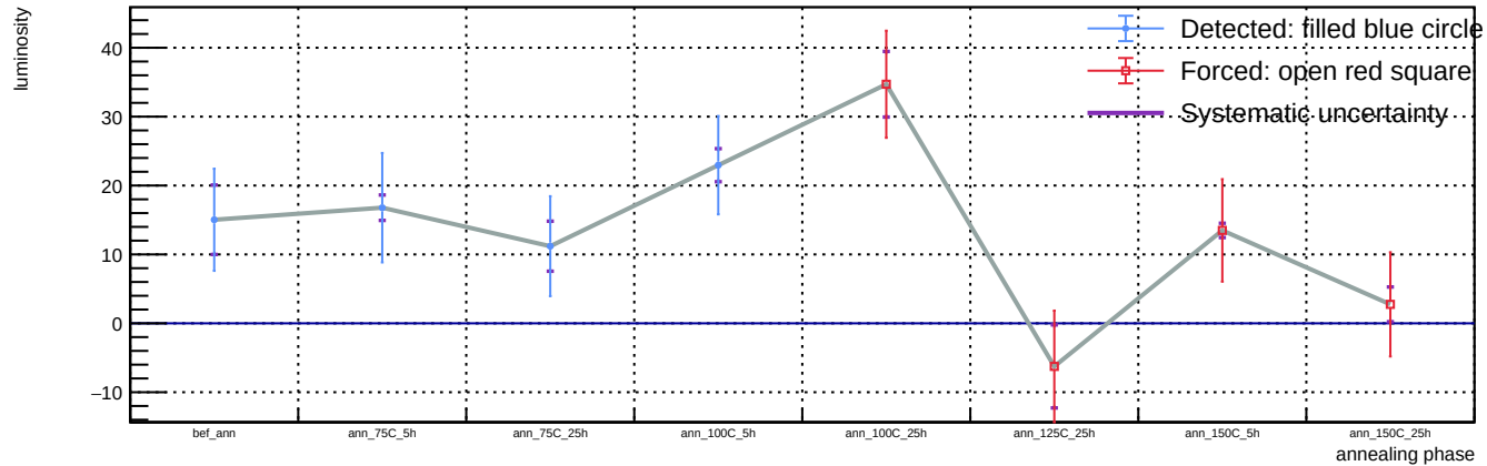
Sensor A1, v = 5 V, representative T = 23 C (max available) - Spot 60: luminosity vs phase
