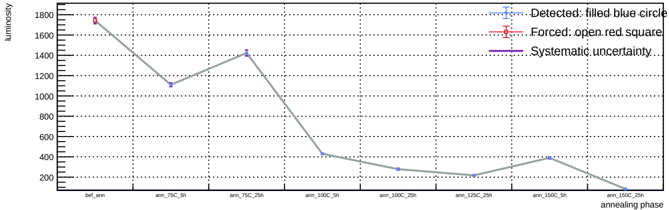
Sensor A1, v = 5 V, representative T = 23 C (max available) - Spot 62: luminosity vs phase
