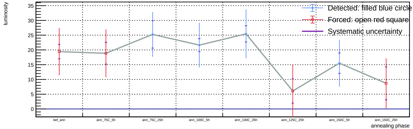
Sensor A1, v = 5 V, representative T = 23 C (max available) - Spot 68: luminosity vs phase
