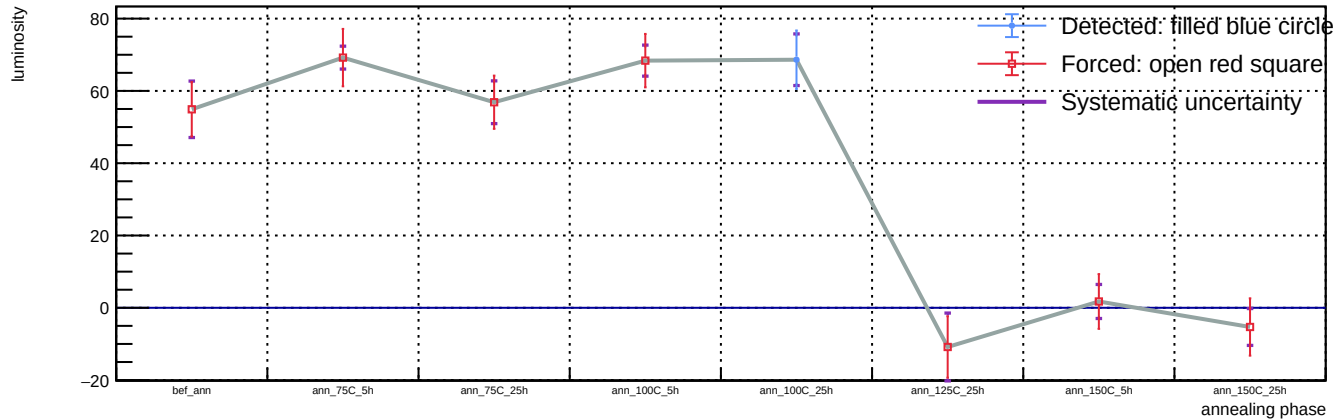
Sensor A1, v = 5 V, representative T = 23 C (max available) - Spot 79: luminosity vs phase
