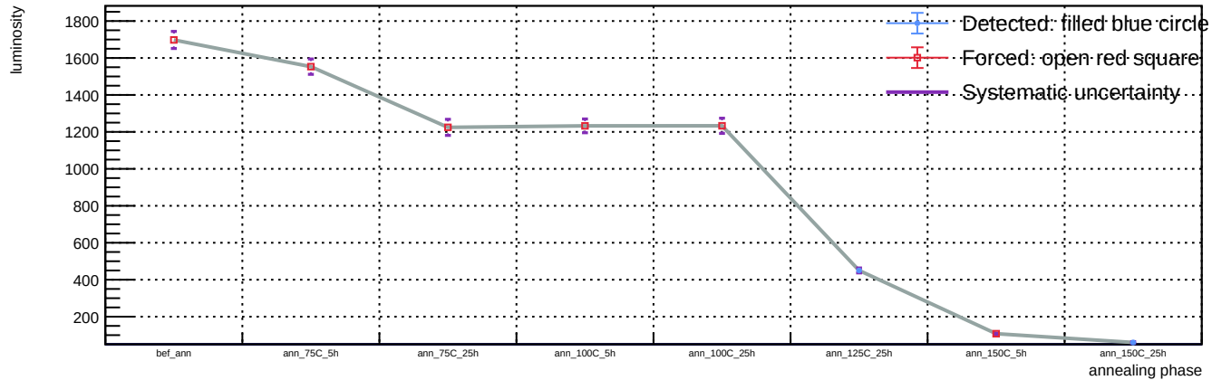
Sensor A1, v = 5 V, representative T = 23 C (max available) - Spot 85: luminosity vs phase
