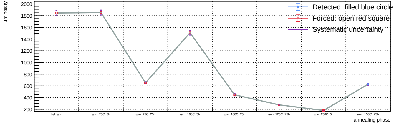
Sensor A1, v = 5 V, representative T = 23 C (max available) - Spot 88: luminosity vs phase
