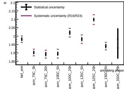
Sensor B1, T = 20 C - Spot 26
