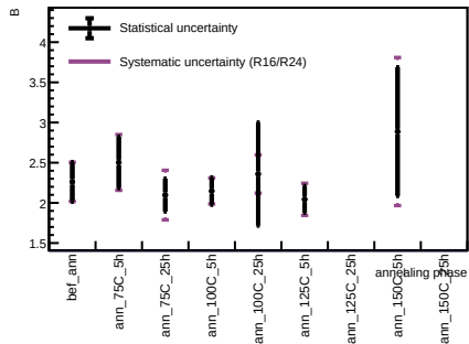
Sensor B1, T = 20 C - Spot 27
