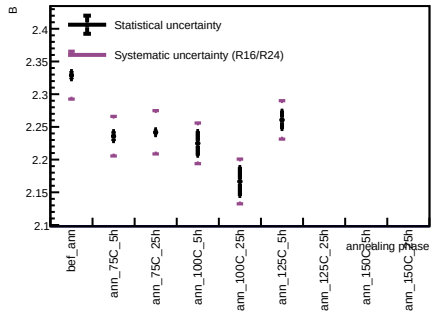
Sensor B1, T = 20 C - Spot 25
