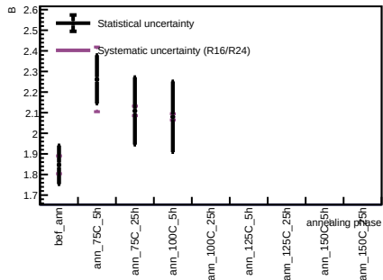
Sensor B1, T = 20 C - Spot 55
