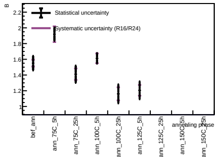
Sensor B1, T = 20 C - Spot 58
