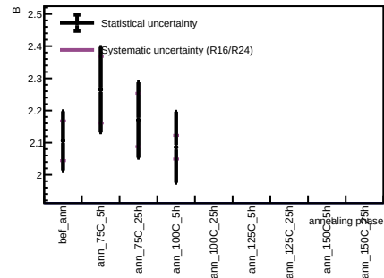
Sensor B1, T = 20 C - Spot 56
