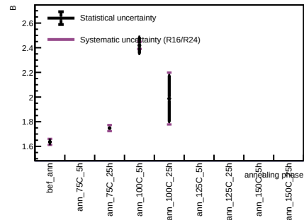
Sensor B1, T = 20 C - Spot 59
