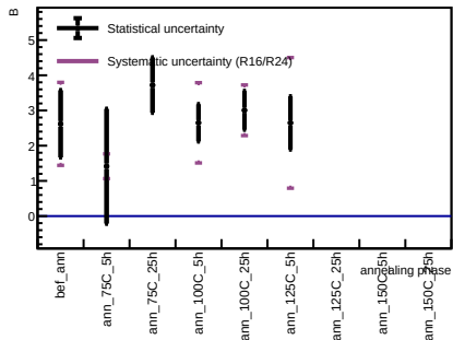
Sensor B1, T = 20 C - Spot 54
