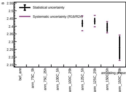
Sensor B1, T = 20 C - Spot 101
