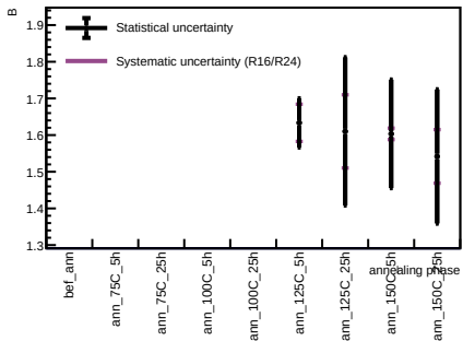
Sensor B1, T = 20 C - Spot 100
