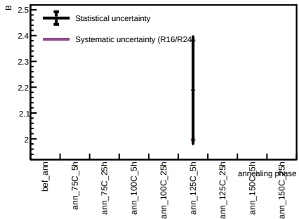
Sensor B1, T = 20 C - Spot 96
