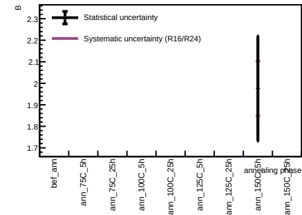
Sensor B1, T = 20 C - Spot 113
