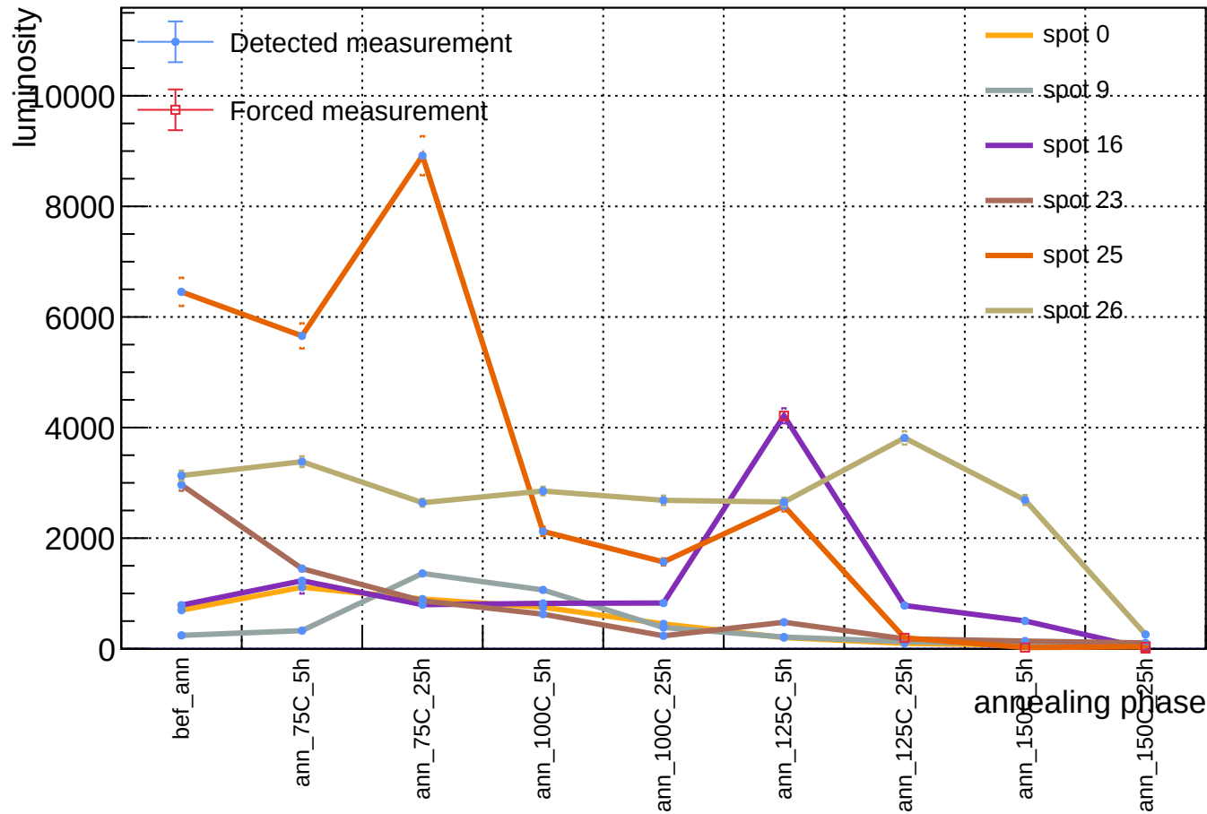
Sensor B1, T = 20 C, representative v = 55.9 V (max available) - luminosity vs phase - order 10^3
