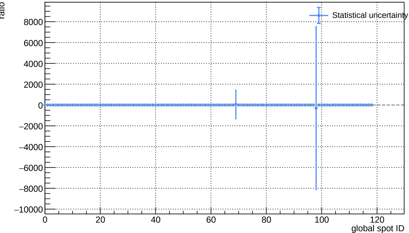
Sensor B1, T = 20 C - L(ann_125C_25h) / L(before_annealing)
