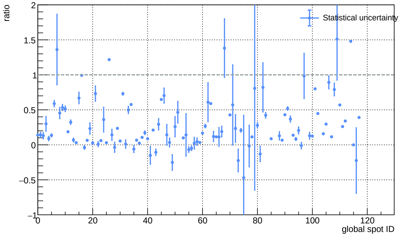
Sensor B1, T = 20 C - L(\text{ann\_125C\_25h}) / L(\text{before\_annealing})
