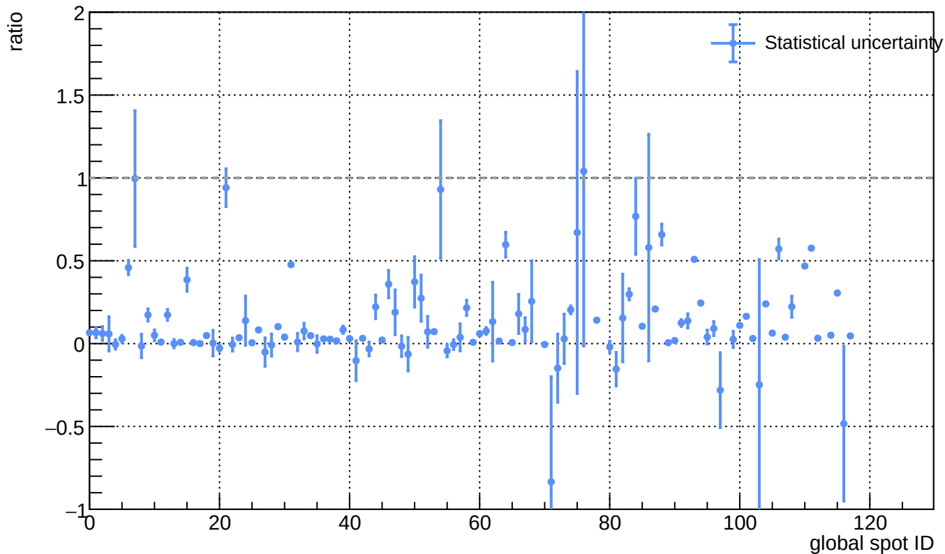
Sensor B1, T = 20 C - L(\text{ann\_150C\_25h}) / L(\text{before\_annealing})
