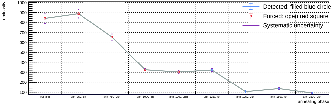
Sensor B1, T = 20 C, representative v = 55.9 V (max available) - Spot 100: luminosity vs phase
