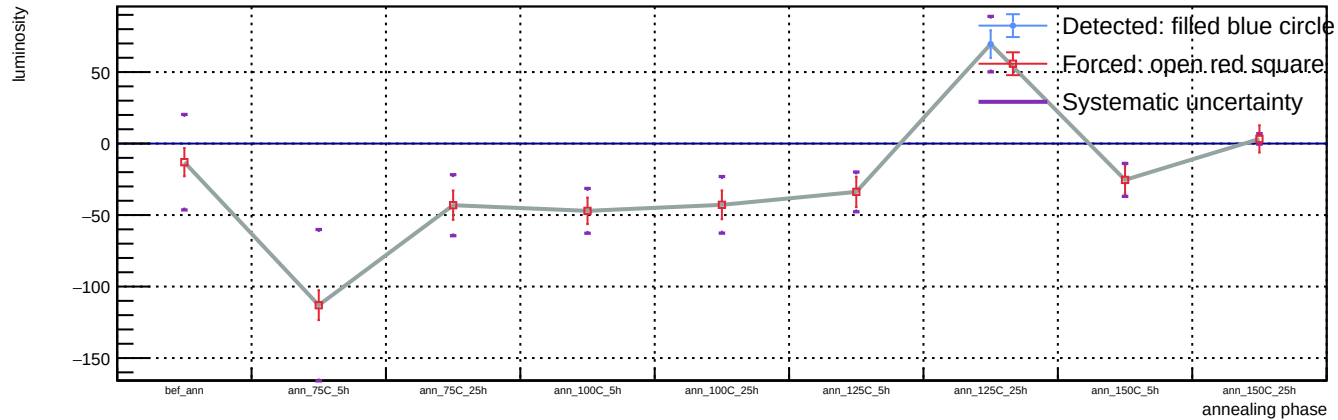
Sensor B1, T = 20 C, representative v = 55.9 V (max available) - Spot 103: luminosity vs phase
