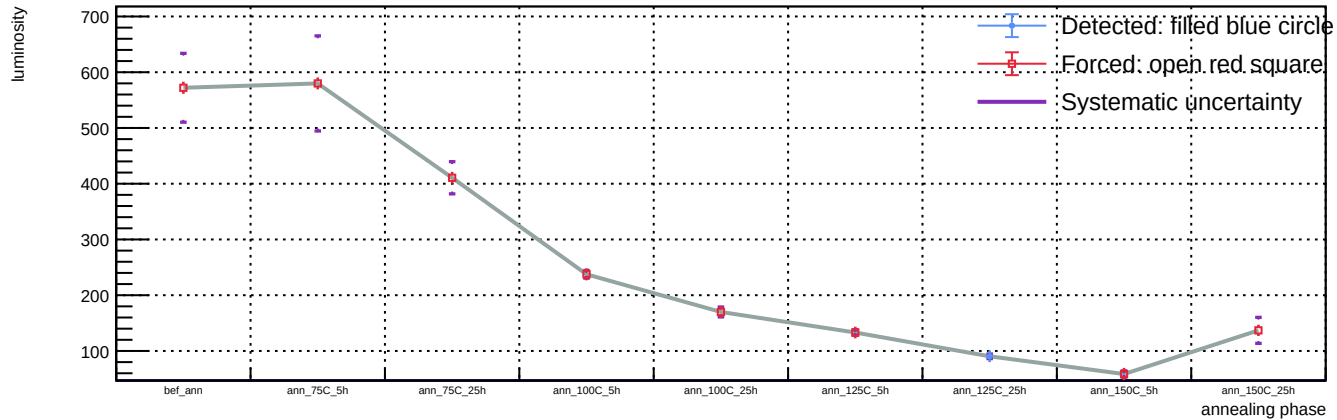
Sensor B1, T = 20 C, representative v = 55.9 V (max available) - Spot 104: luminosity vs phase
