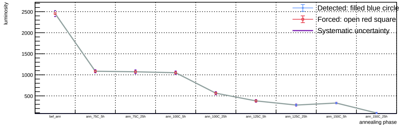
Sensor B1, T = 20 C, representative v = 55.9 V (max available) - Spot 107: luminosity vs phase
