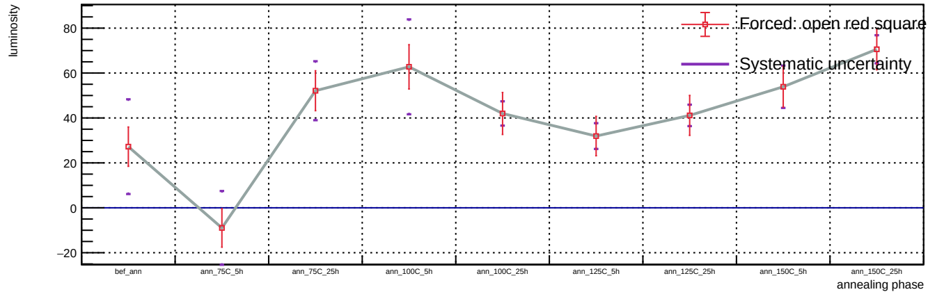
Sensor B1, T = 20 C, representative v = 55.9 V (max available) - Spot 109: luminosity vs phase
