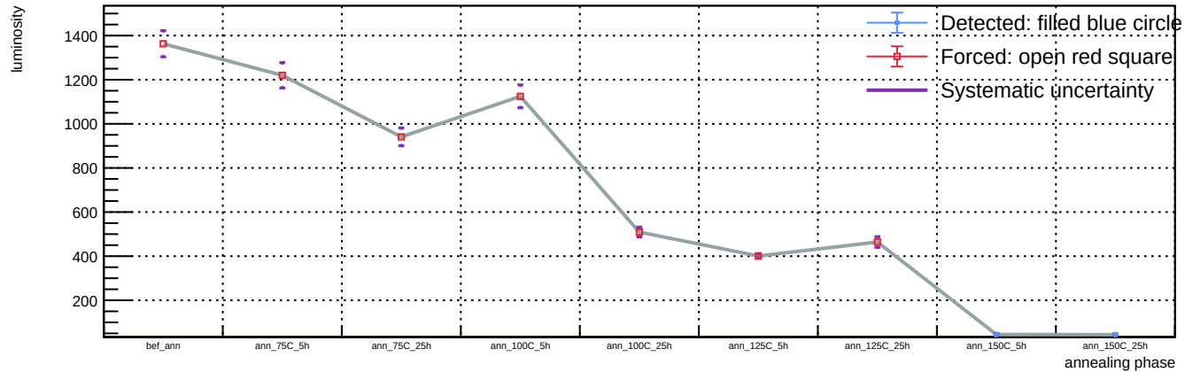
Sensor B1, T = 20 C, representative v = 55.9 V (max available) - Spot 112: luminosity vs phase
