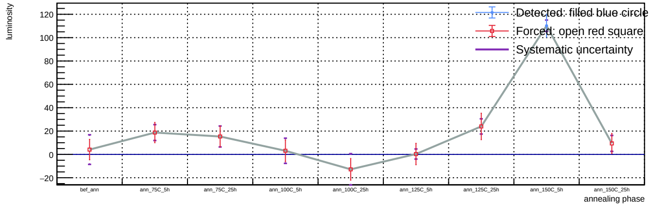
Sensor B1, T = 20 C, representative v = 55.9 V (max available) - Spot 113: luminosity vs phase
